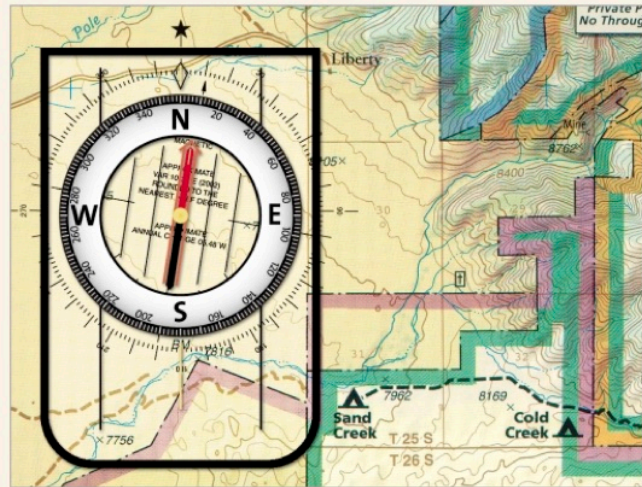
Set the compass's declination for your area. Note that the magnetic north and declination are aligned, (10.5° E in this example), while true north is at the top of the page and map.
