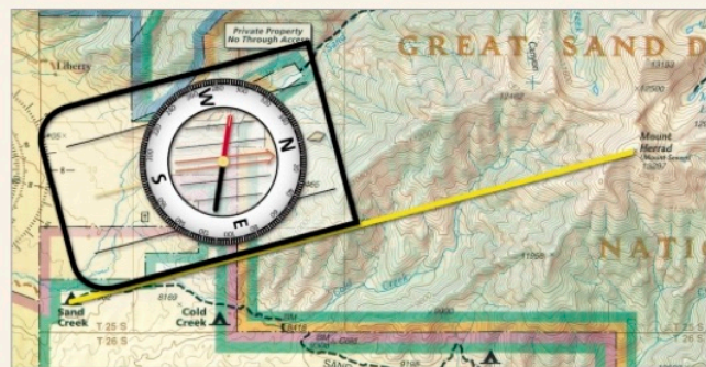
Next, from your location (Sand Creek Campground in this example) mark a line on the map to your point of interest (Mount Herrad in this case) and lay the compass along this line in the travel direction. (The straight edge of the compass, especially one with a folding cover, may span the map distance without needing to draw a line). Without a map aim the compass as precisely as possible by sight. Note the difference now between magnetic north red needle and the orienting arrow.
