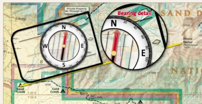
Now turn the azimuth ring so the orienting arrow and the compass needle are aligned. The value that the index pointer shows is your bearing to that location (75° East Northeast in this example).
