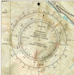
Compass Rose with no declination deviation and one with an 11° East declination on a map. True north in both instances is at the top of the page.
