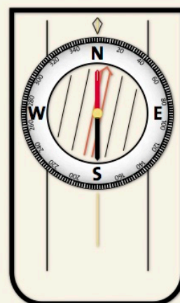
Basic compass with declination adjustment of 12 degrees East. Orienting arrow is adjusted for magnetic north. True north and magnetic north are separated by 12 degrees in this example.
